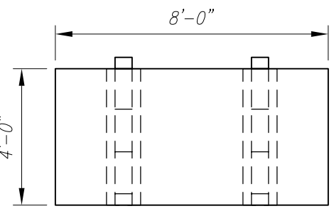
PIECE FRONT ELEVATION
