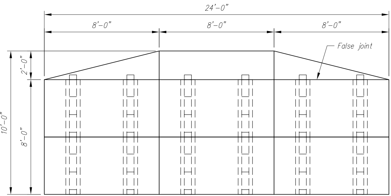
LAYOUT FRONT ELEVATION
