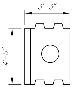
PIECE SIDE ELEVATION
